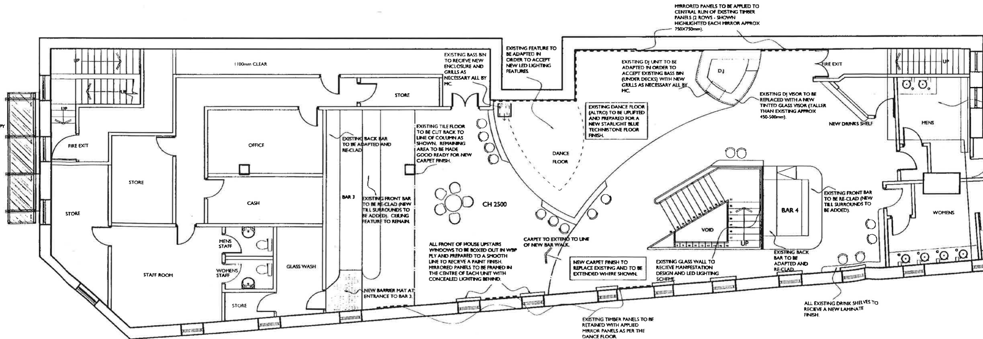
FIRST FLOOR PLAN - SCALE 1:100
