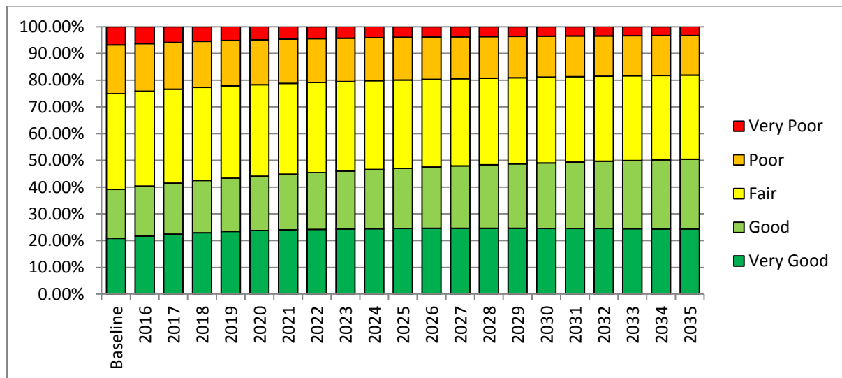
Figure 1: Worst-first Strategy
